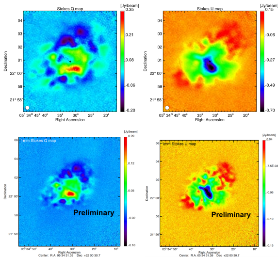
Fig. 28. From left to right Stokes Q and U maps obtained with NIKA at 150 GHz (top) Ritacco, A. et al. (2018) and NIKA2 at 260 GHz (bottom) (Ritacco, A. et al. 2020).
