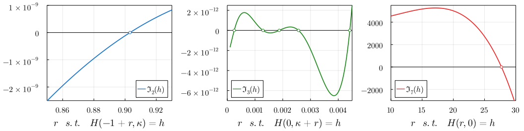
Fig. 6. Abelian integrals \mathfrak{J}_2, \mathfrak{J}_3, \mathfrak{J}_7 in Li, Liu and Yang’s system (7.4) with the parameters of Theorem 7.2, having 1, 5 and 1 zeros, respectively.
