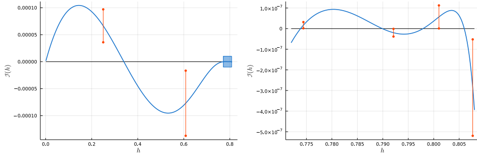
FIGURE 2. Rigorously computed interval enclosures of \mathfrak{I}(h) on small ovals, for h \in \{0.25, 0.6084, 0.7744, 0.7921, 0.801025, 0.80766169\} , proving the existence of 5 zeros. The right plot is a zoom of the blue box in the left plot.
