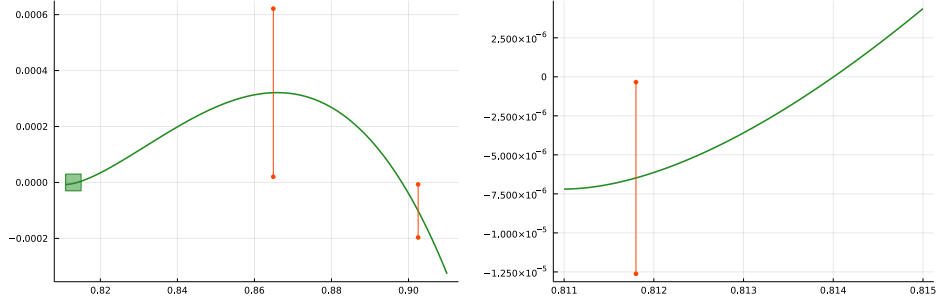
FIGURE 3. Rigorously computed interval enclosures of \mathfrak{I}(h) on big ovals, for h \in \{0.811801, 0.8649, 0.9025\} , proving the existence of 2 zeros. The right plot is a zoom of the green box in the left plot.
