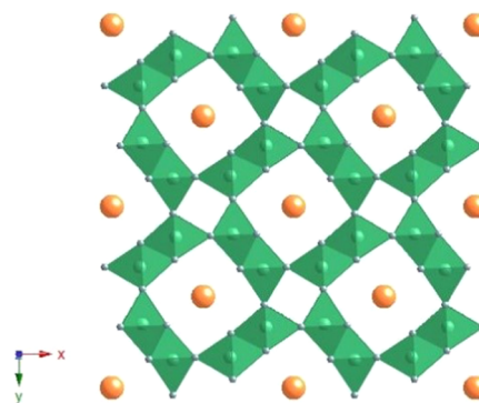
Figure 1. Schematic drawing of the crystal structure of hollandite oxide ( K_xMnO_2 ). Color code: K, orange; Mn, green; and O, gray.
