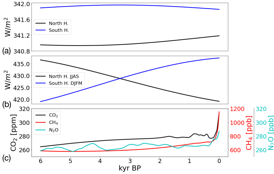
Fig. 1 Evolution of the incoming solar radiation [W/m^2] at the top of the atmosphere and trace gases in the last 6000 years (0 kyr BP = 1950). Panel a: annual mean incoming solar radiation averaged in the Northern Hemisphere (NH) [0-90N] and Southern Hemisphere (SH) [0-90S]. Panel b: solar radiation averaged for the months of June to September (JJAS) in the NH and December to March (DJFM) in the SH. Panel c: annual mean of CO_2 [ppm], CH_4 [ppb], and N_2O [ppb] averaged globally. Both radiation and trace gases forcing are updated yearly. Details on the forcing factors can be found in Braconnot et al. (2019b).
