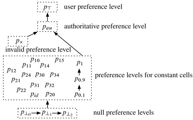
Fig. 4: Partial order \preceq_{\mathbf{P}} on preference levels used in our running example. Arrows between preference levels denote \prec_{\mathbf{P}} (strictly less). No arrow means incomparable. Arrows between dotted boxes mean that all levels in one box are strictly less preferred than those in the other box.
