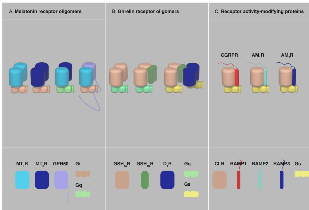
Fig. 7. Oligomerization of GPCRs with orphan GPCRs, truncated GPCRs and RAMPs. (A) Homomers and heteromers of MT 1 R, MT 2 R and GPR50. MT 2 R preferentially exists as a heteromeric complex with MT 1 R and MT 1 R-MT 2 R heteromerization drives a change in the preference of G protein subtype coupling, from Gi to Gq. The long CT of GPR50 significantly alters MT 1 R-Gi protein signaling in the MT 1 R-GPR50 heteromer (see text). (B) GHS1aR forms homomers and oligomerizes with its non-functional truncated isoform GHS1bR to form homomers and heteromers. One of the properties of the GHS 1a R-GHS 1b R oligomers is the facilitation of an additional interaction with the D 1 R, leading to a change in the preference of G protein subtype coupling of GHS 1a R, from Gq to Gs. (C) The single TM domain proteins RAMP1, RAMP2 and RAMP3 associate with CLR and form the Gs protein-coupled receptors CGRPR, AM 1 R and AM 2 R, respectively, determining the ligands potentially binding to CLR.
