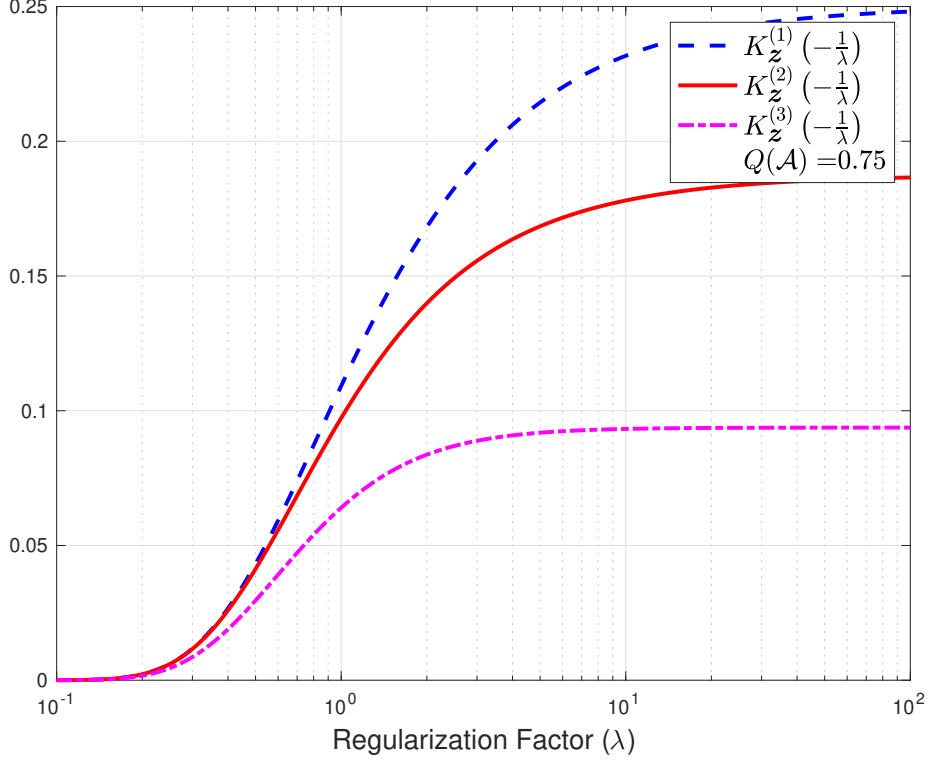
Figure 1: Mean K_{Q,z}^{(1)}(-\frac{1}{\lambda}) , variance K_{Q,z}^{(2)}(-\frac{1}{\lambda}) , and third central moment K_{Q,z}^{(3)}(-\frac{1}{\lambda}) of the empirical risk in Example 6.1, with Q(\mathcal{A}) = \frac{3}{4}
