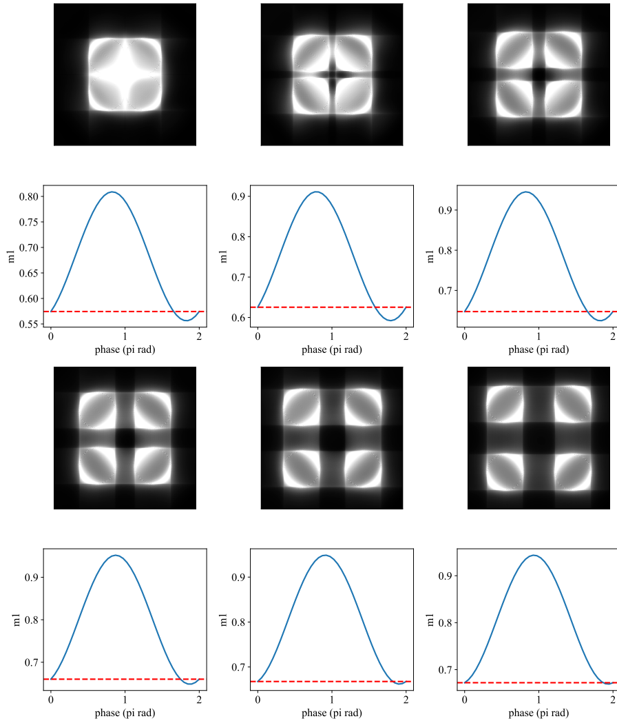
Figure 2: Dependence of PWFS tilt angle on m_1 vs. additive piston phase curve (as in Fig. 1b). The pupil intensity image for the additive piston phase at which m_1 is minimized is shown above each corresponding curve. All images are displayed on the same relative contrast scale.
