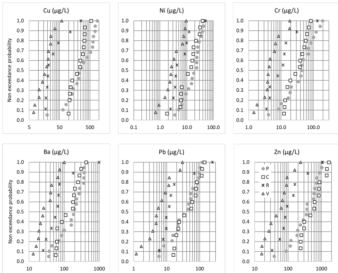
Figure 3. Non-exceedance probability distributions of the total EMCs (µg/L) for Cu, Ni, Cr, Ba, Pb and Zn. P = Paris, C = Compans, R = Rosny-sous-Bois and V = Villeneuve-le-Roi.
