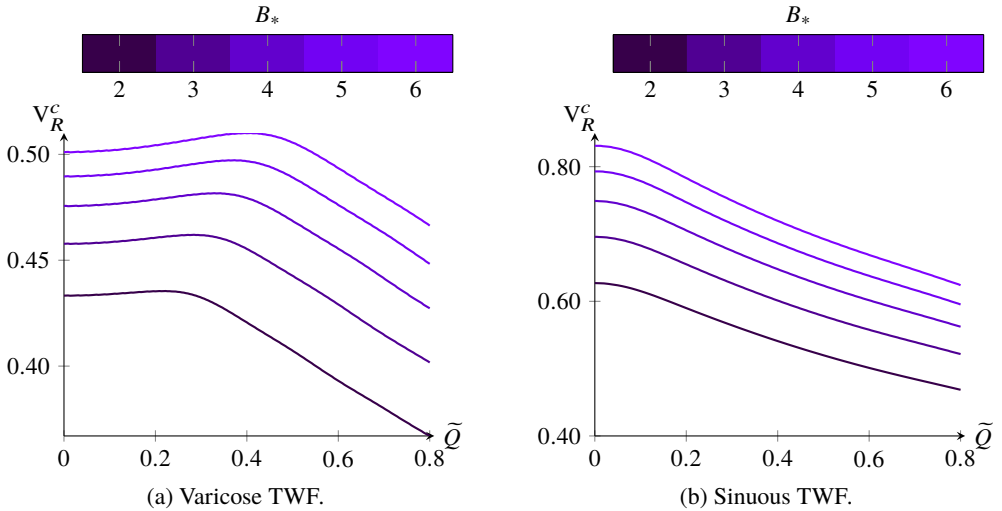
Figure 22: Critical V_R^c for TWF modes for different B_* . The other parameters are: Wo = 20 , Re = 10000 and d_* = 0 .
