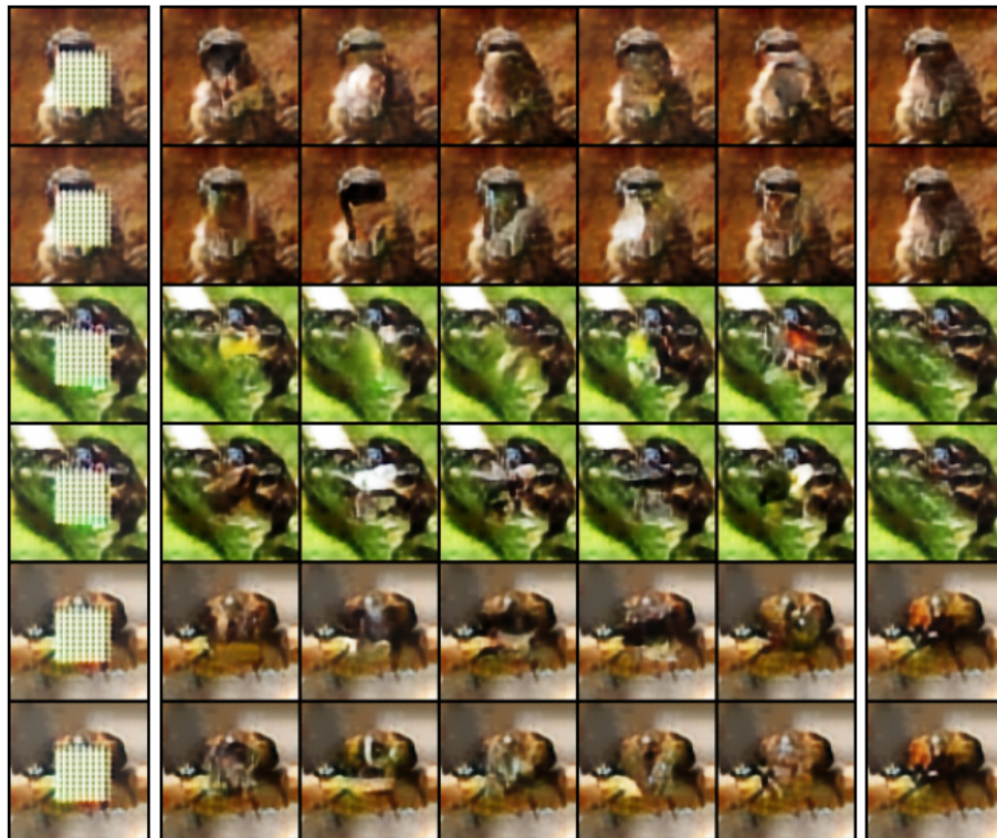
Figure 5: Conditional sampling with centered mask: for each of the 3 different images, samples from our diffusion are on top and from PixelCNN on the bottom. For each row: the image on the left is the VQVAE masked reconstruction, the image on the right is the full VQ-VAE reconstruction. Images in-between are independent conditional samples from the models.
