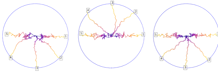
Figure 11: Three independent sampling of X using a trained diffusion bridge, with fixed q_1 = 0, q_5 = 4 . The three corresponding sequences are (0, 7, 6, 5, 4) , (0, 1, 2, 3, 4) , (0, 7, 6, 5, 4) all valid sequences.
