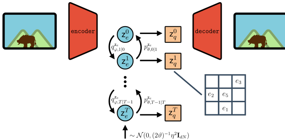
Figure 1: Our proposed architecture, for a prior based on a Ornstein-Uhlenbeck bridge. The top pathway from input\ image to z_e^0 , to z_q^0 , to reconstructed\ image resembles the original VQ-VAE model. The vertical pathway from (z_e^0, z_q^0) to (z_e^T, z_q^T) and backwards is based on a denoising diffusion process. See Section 3.2 and Algorithm 2 for the corresponding sampling procedure.
