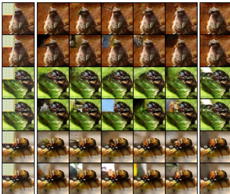
Figure 6: Conditional sampling with top left mask: for each of the 3 different images, samples from our diffusion are on top and from PixelCNN on the bottom. For each row: the image on the left is the VQVAE masked reconstruction, the image on the right is the full VQ-VAE reconstruction. Images in-between are independent conditional samples from the models.
