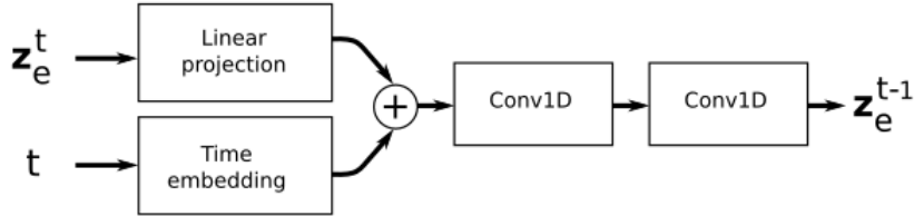
Figure 9: Graphical representation of the neural network used for the toy dataset.
