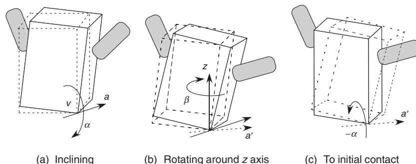
Figure 3 Sequence of pivot motion of a box object: (a) inclining; (b) rotating around z axis; and (c) to initial contact.
