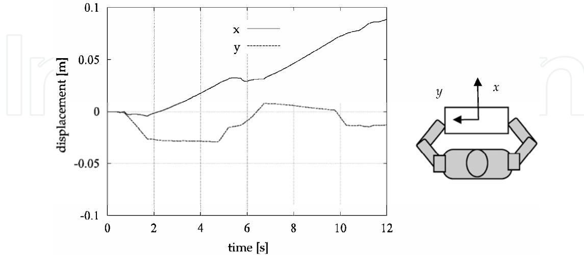
Figure 9. Simulation result of displacement of the center of mass of the manipulated object in x and y directions shown at right-hand side
