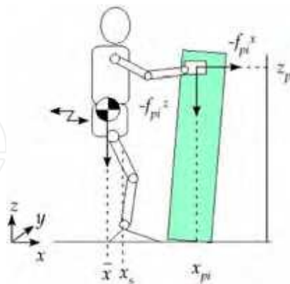
Figure 7. Body-balancing by moving waist position. According to the contact forces at the hands, the humanoid robot adjusts its waist position to maintain the "static balancing point" at the center of the support polygon
