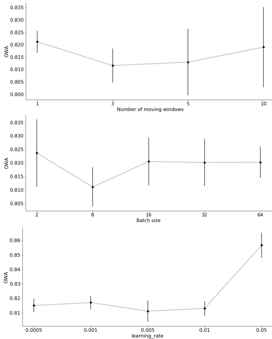
Figure 12: OWA for the hermes-tbats model on the M4 weekly dataset depending on 3 parameters used during the RNN training: Number of moving windows per time series, the batch size and the learning rate. For each parameter, 10 models with different seeds have been trained. The mean and the standard deviation are represented with a point and a vertical. (Top) Result of the HERMES model depending on the number of windows provided per time series to the RNN corrector. (Middle) Result of the HERMES model depending on the size of the batch size. (Bottom) Result of the HERMES model depending on the learning rate of the optimizer.
