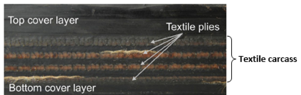
Figure 1. Rubber-textile composite conveyor belt.
