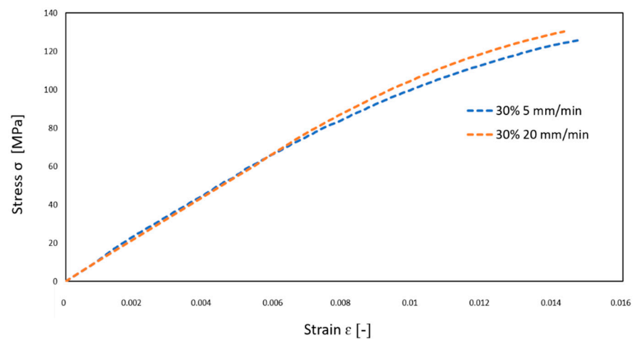
Figure 5. Conventional stress–strain diagrams of 30% GF/PBT tested at 5 and 20 mm/min.
