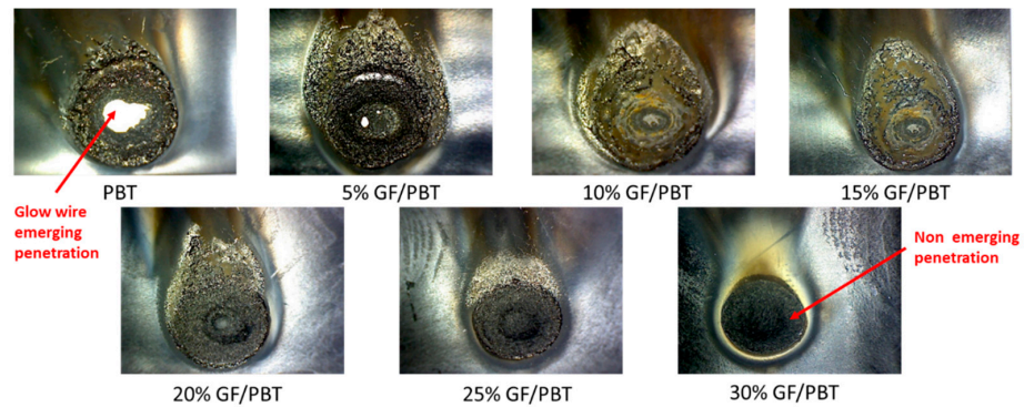
Figure 13. Appearance of the ignited surface vs. GF reinforcement rate.
