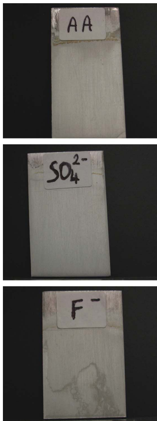
Fig. 8. Photographs of aluminum plates after the anodization treatment (AA) and after corrosion experiments in the presence of some electrolyte solutions at 0.01 \text{ mol L}^{-1} concentration.
