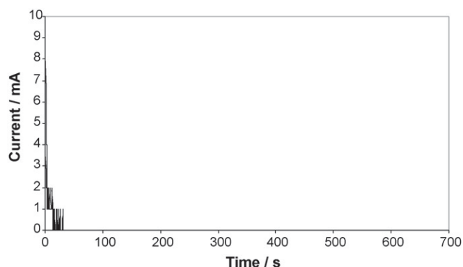
Fig. 7. Variation of the current intensity as a function of time during application of a 8 V/MSE working potential on plates I in the presence of cosmotope anions at 0.01 \text{ mol L}^{-1} concentration.
