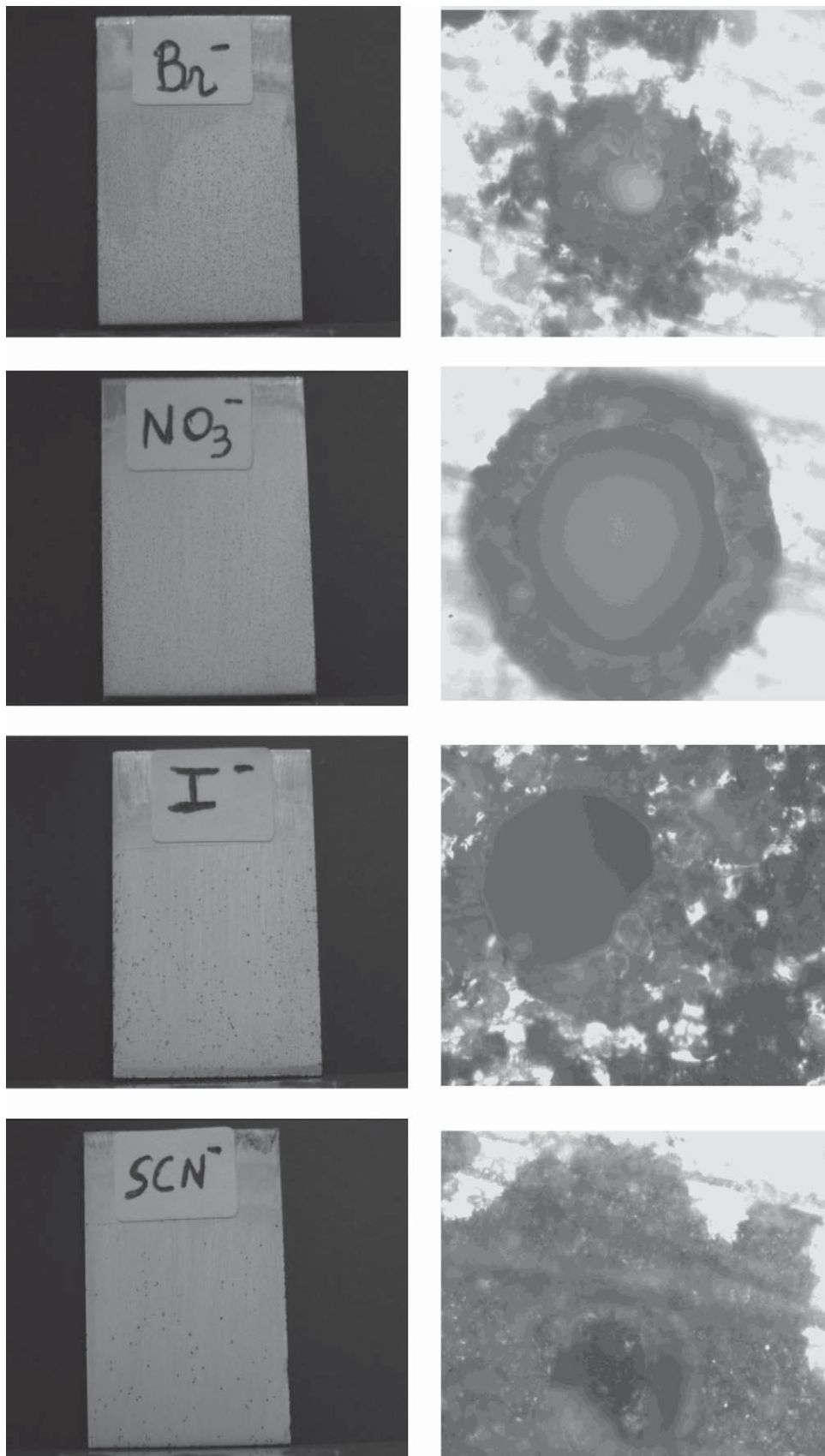
Fig. 6. Photographs (on the left side) and micrographs (on the right side, magnification ×50) of plates I after corrosion experiments in the presence of some electrolyte solutions at 0.01 molL -1 concentration.
