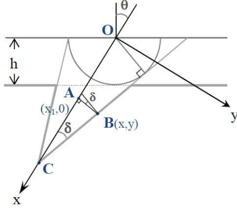
Figure 1 : Geometric representation of an etched track with dip angle \theta in the case of a conical in shape model (i.e. both V_b and V_t are constant).
