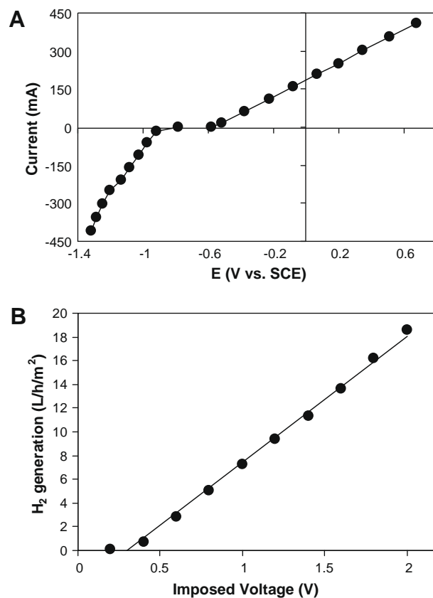
Fig. 3. Characterisation of a 25 L pilot MEC with 0.5 M phosphate pH 8.0 in the cathode compartment and seawater in the anode compartment. (A) Current–potential curves recorded by imposing successive cell voltages step by step; (B) hydrogen generation rate as a function of the cell voltage.
