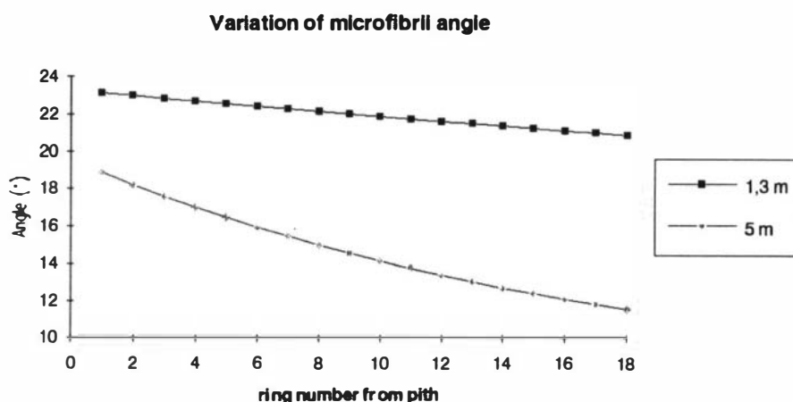
Graph 3 : Radialvariation of the microfibrill angle at the two heights of sampling.
