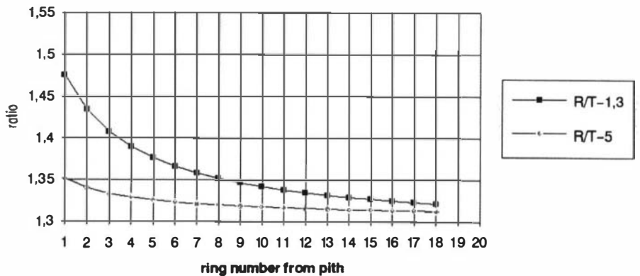
Graph 2 : Trend of radial to tangential diameters ratio
