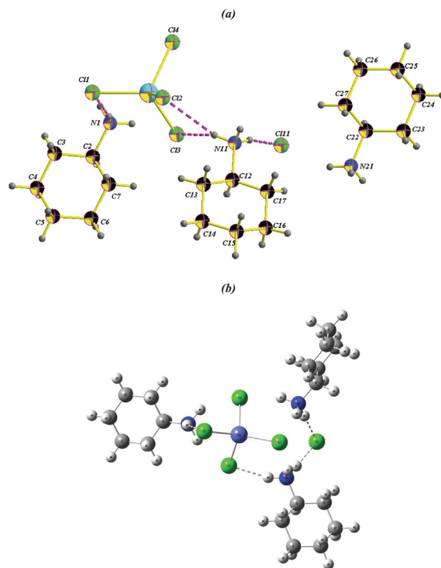
Fig. 1. Ortep structure (a) with atom numbering and optimized molecular geometrical structure (b) of (C_6H_{14}N)_3[CoCl_4]Cl .
