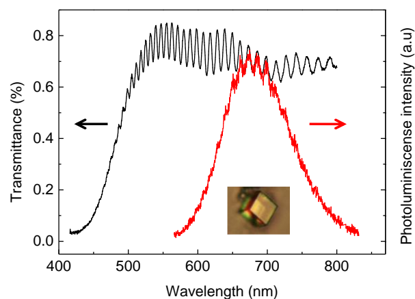
Figure 4. OT (black) and PL (red) spectra of the crystal shown in the inset.
