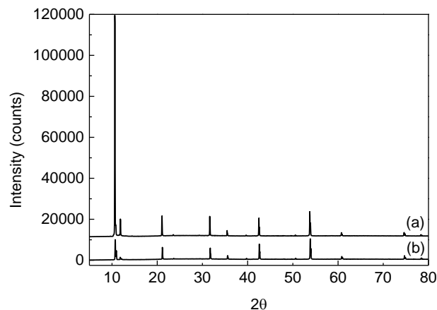
Figure 2. X ray patterns of a set of single crystals of MC before (a) and after optical studies (b).
