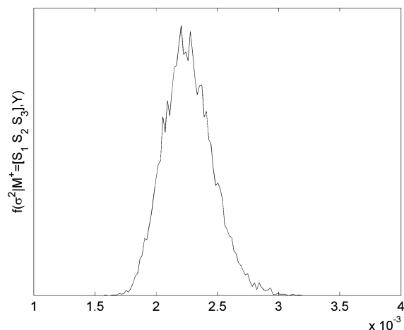
Fig. 5. Posterior distribution of the estimated variance \sigma^2 .
