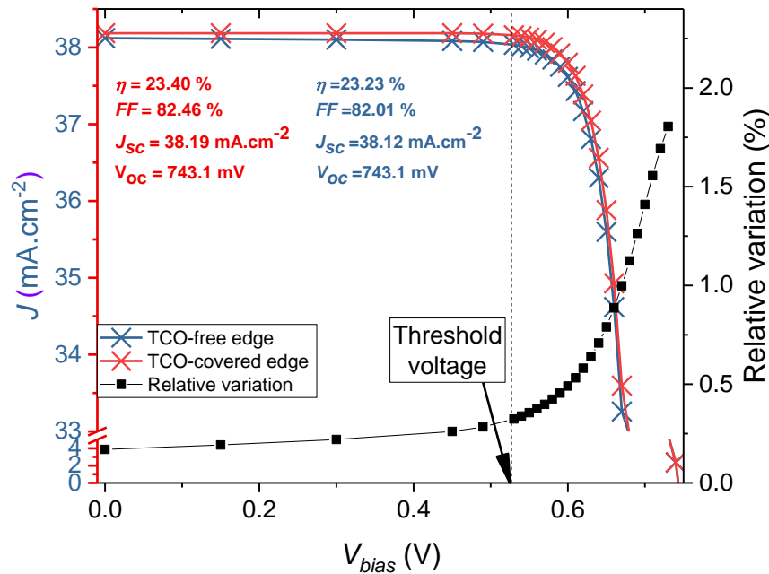
Figure 2: Simulated I(V) curves for M6 full size cells with rear TCO-free edges (blue) or rear TCO-covered edges (red) with edge D_{it}=0\text{ cm}^{-2} . The I(V) parameters of each cells are given with the same colour code. The relative variation between the two curves is plotted in black.
