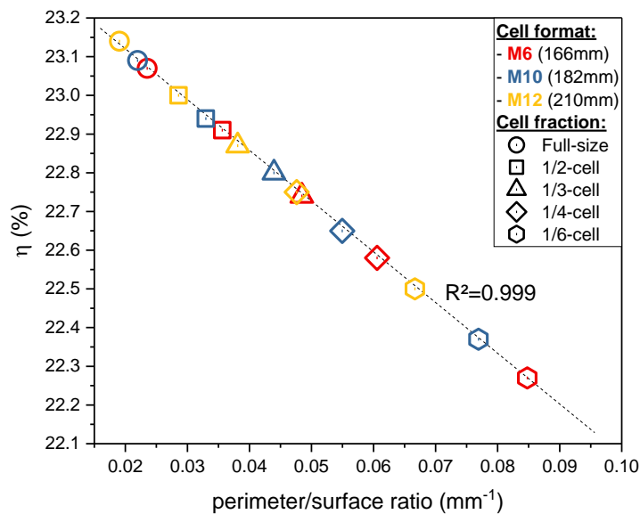
Figure 9: Cut-cells efficiency as a function of their perimeter/surface ratio. Edge D_{it}=3 \times 10^{10} \text{ cm}^{-2} for native edge, D_{it}=10^{14} \text{ cm}^{-2} for cut edge. Since \alpha -type and \beta -type cells have the same performance in the as-cut condition, only the performances of \alpha -type cells are given here.
