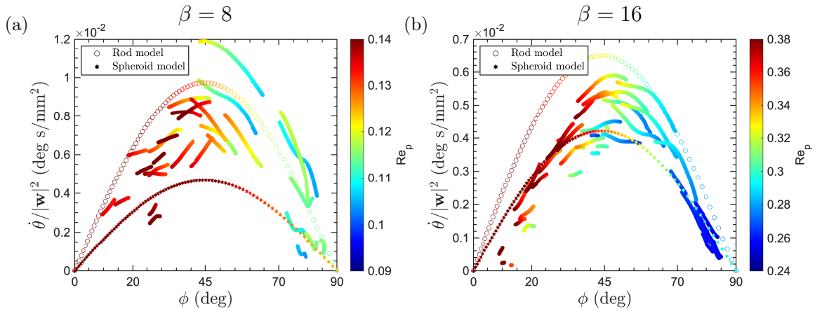
FIG. 5. The measured angular velocity, \dot{\theta} , divided by |\mathbf{w}|^2 , color coded by the local value of Re_p . The predictions of Eq. (9) are shown for the spheroid model and for the slender-rod model, as indicated by the legend. Panel (a) corresponds to \beta = 8 , and (b) to \beta = 16 .
