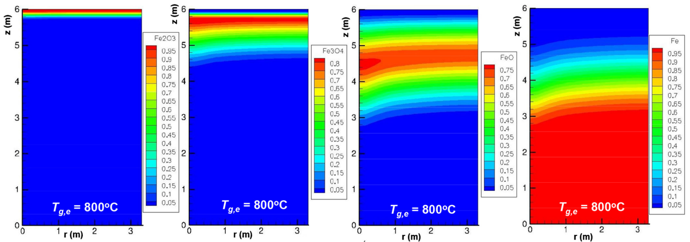
Fig. 11. Calculated solid mass fractions in a shaft furnace fed with \text{H}_2 at 800^\circ\text{C} . The symmetry axis is on the left-hand side of each map, and the wall is on the right-hand side. The main gas inlet is at the wall near the bottom of the reactor.
