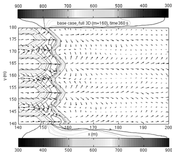
Fig. 2: Local “down-fire” winds, seen from above. The prevailing wind is blowing from left to right in direction x. The coloured contour lines represent gas isotherms (temperature in Kelvin). The vectors represent the horizontal dimension of local wind speed.
