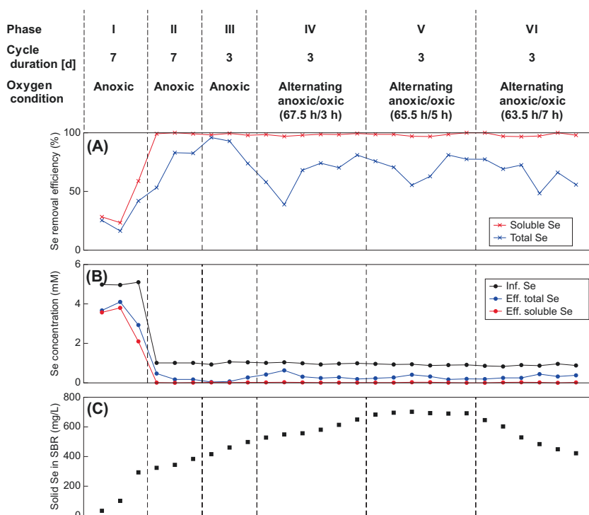
Fig. 3.16 Se removal performance of the sequencing batch reactor: (a) Se removal efficiencies; (b) Se concentrations in the influent and effluent; and (c) solid Se in the reactor. (Adapted from Zhang et al. 2019a)
