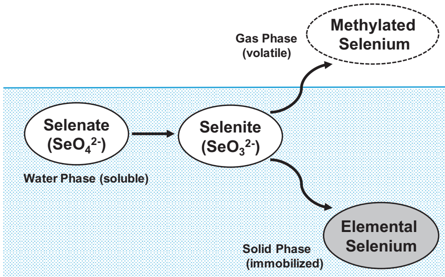
Fig. 3.15 Microbial selenium metabolism enabling the removal of soluble Se as selenate and selenite from the water phase. Selenate reduction into selenite proceeds mainly under anoxic conditions; selenite volatilization occurs mostly under aerobic conditions, while selenite reduction into elemental Se proceeds under both aerobic and anoxic conditions
