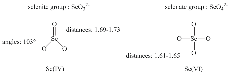
Scheme 3.1 Structures of selenite and selenate oxyanions, showing distances between Se and O atoms
