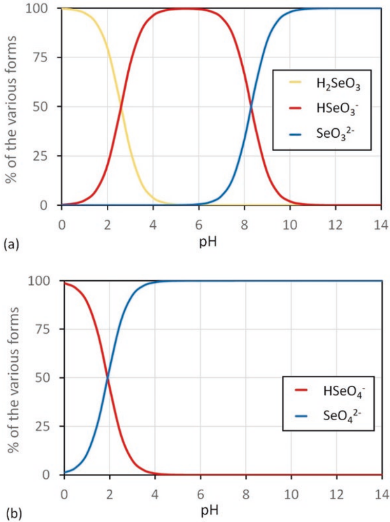
Fig. 3.13 Distribution diagrams of the various forms of a) Se(IV) and b) Se(VI)
