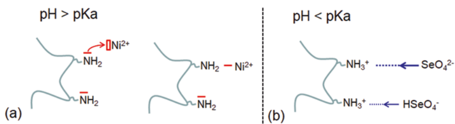
Fig. 3.11 (a) Complexation mechanism with metal ions, and (b) electrostatic attraction with oxyanions of Se(VI) by amine groups of polymers
