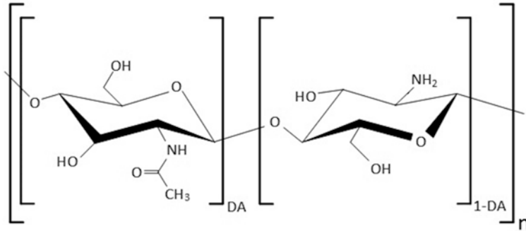
Fig. 3.12 Chitosan molecule. DA: degree of acetylation
