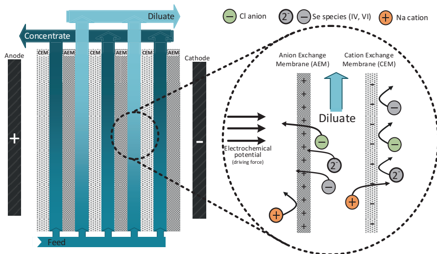
Fig. 3.9 Principle of an electrodiolysis process. (Source: Mehran Aliaskari, Eggenstein-Leopoldshafen, Germany)
