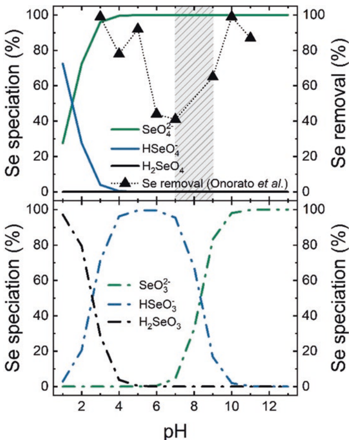
Fig. 3.10 Speciation of selenium VI (top) and IV (bottom) over pH 1 to 13 and removal of selenium VI, adapted from Onorato et al. (2017); electric potential 12 V; feed salinity 5.3 g/L; membranes Neosepta CMX-SB & AMX-SB, Tokuyama Soda Ltd., Japan; the highlighted pH range shows the real pH of sample water used which was then modified by adding HCl and NaOH)
