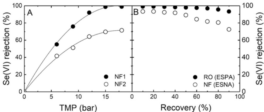
Fig. 3.8 Rejection of Se(VI) with nanofiltration/reverse osmosis membranes as a function (a) the transmembrane pressure (TMP) and (b) the recovery (source: (a) adapted from Malhotra et al. (2020): Se(VI) 1600 \mu\text{g/L} and pH 8; (b) adapted from Chung et al. (2010): S(VI) 326 \mu\text{g/L} , pH 7.2 and pressure 8 bar)
