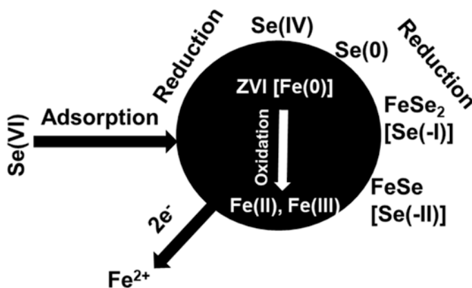
Fig. 3.4 Se(VI) adsorption and subsequent reduction to Se(IV), Se(0), Se(-I), and Se(-II) by zero-valent iron. (Adapted from Shrimpton et al. 2015)
