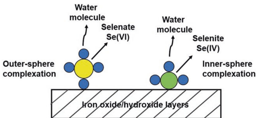
Fig. 3.5 Selenate and selenite adsorption onto iron oxide and hydroxides. (Adapted from Hayes 1987)
