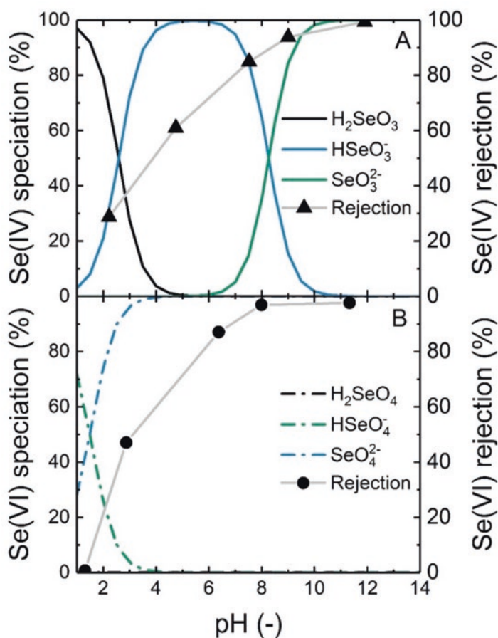
Fig. 3.7 Speciation of selenium (Se) and its rejection with laboratory-made TFN membrane, adapted from He et al. (2016a, b); speciation of Se(IV) and Se(VI) was calculated at 25°C and CO_2 partial pressure of 3.9 \cdot 10^{-4} bar, by using the software MINTEQ v.3.1, KTH, Sweden
