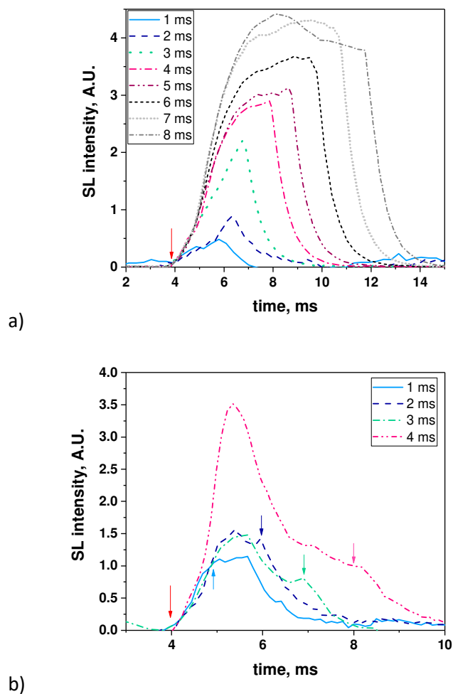
Fig. 1: Evolution of the SL intensity during t_{on} , for various t_{on} values, Ar-saturated water, 362 kHz, 10°C, a) P_{ac} = 48 W, ( V_{PMT} = 600 V for 3-8 ms, 1000 V for 1-2 ms), b) P_{ac} = 4.4 W ( V_{PMT} = 1000 V) (curves obtained at higher t_{on} are presented in Fig. 2SI in Supporting Information) (for each curve, the second arrow indicates the end of the US pulse).
