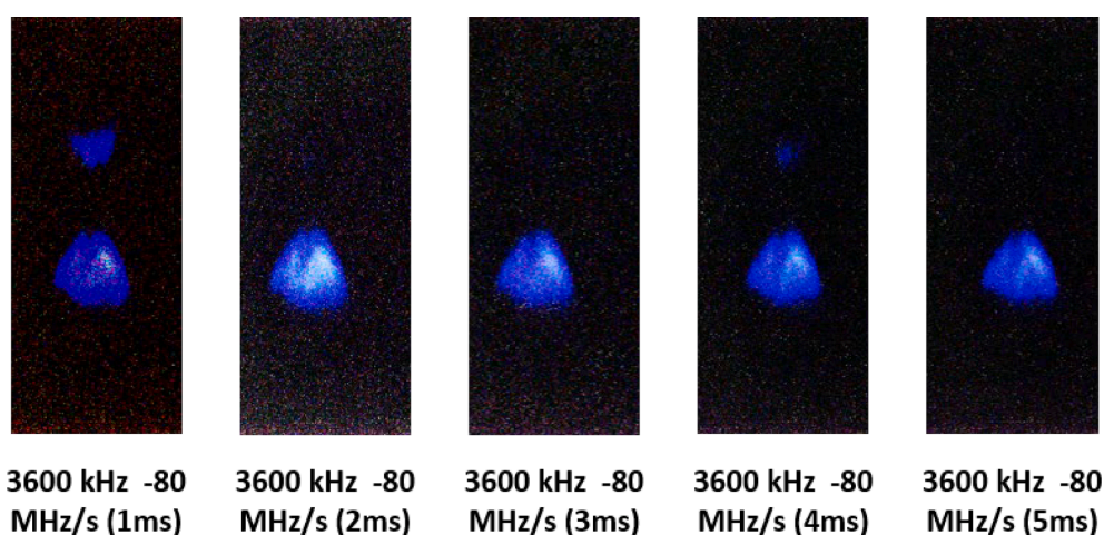
Fig. 3. SCL imagery with luminol (0.01 M, pH = 10.8, \text{Na}_2\text{CO}_3 ), Ar-20% \text{O}_2 , iso 3200, 1-minute duration, using a Canon EOS 100 D camera.
