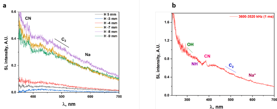
Fig. 8. (a) SL emission spectra of HIFU in wobbling mode, in 1 M NaCl + 3.7 mM 2-propanol under Ar-15.5%O 2 -2.2%N 2 at 3600–3520 kHz (1 ms) at different heights H. (b) SL emission spectra of HIFU in wobbling mode, in 1 M NaCl + 3.7 mM 2-propanol under Ar-15.5%O 2 -2.2%N 2 at f = 3600\text{--}3520 kHz, -80 MHz/s (1 ms), merged with the corresponding spectra using high-pass filter 320 nm.
