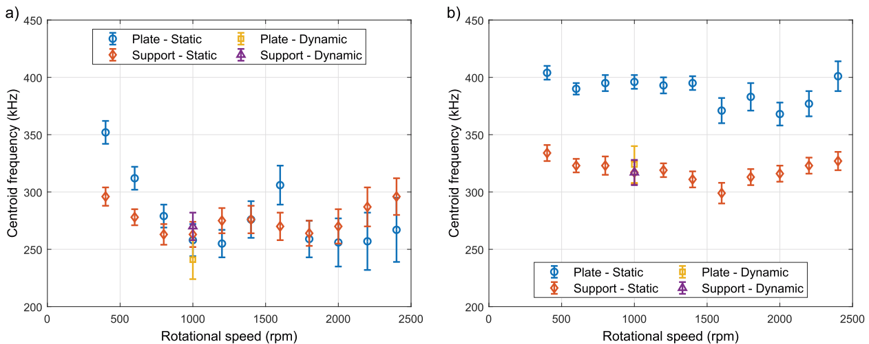
Fig. 18. Evolution of centroid frequency as a function of the rotational speed: a) AA7075-T6 and b) AA6082-T6.
