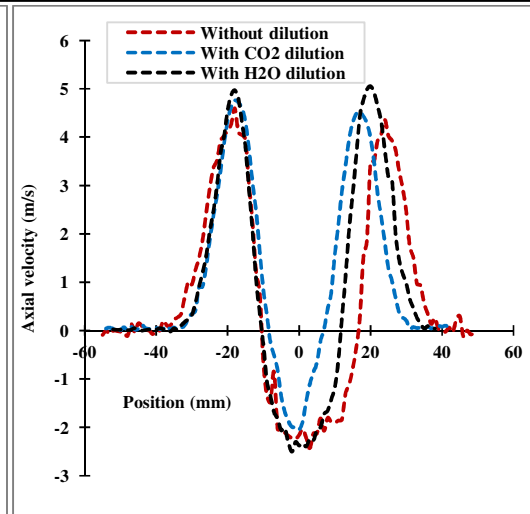
Figure 7. Comparison of profiles of axial velocity at z= 30 mm with and without dilution.
