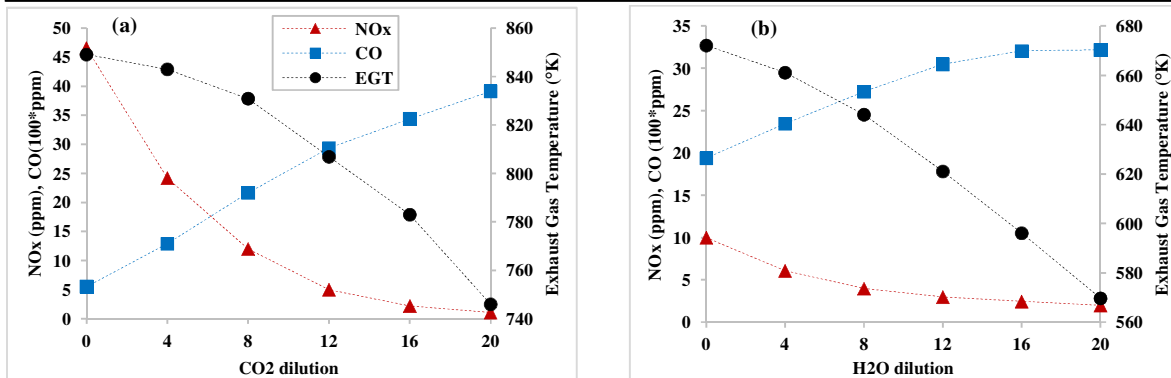
Figure 2. NOx, CO and EGT: (a): as function of CO 2 , at 25%O 2 , \phi=0.8 and Sn=1.4. (b): as a function of H 2 O dilution at 21%O 2 , \phi=0.8 and Sn=1.4
