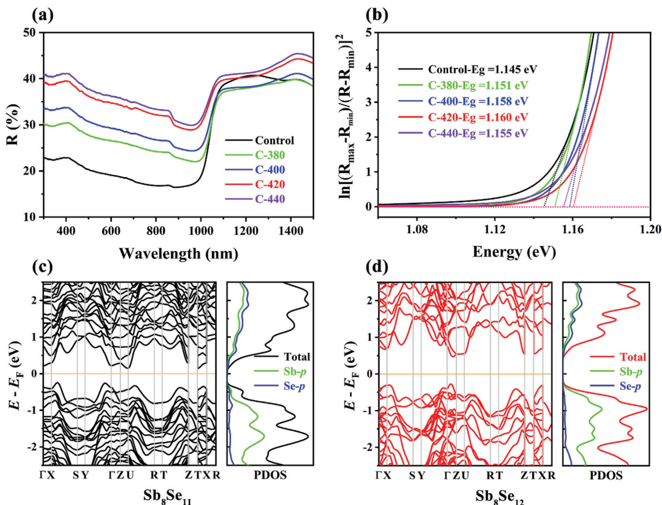
Figure 3. Optical characterizations of the Sb 2 Se 3 thin films: a) Reflection spectra, b) Plots of \ln[(R_{\max} - R_{\min})/(R - R_{\min})]^2 versus Energy, used to obtain direct bandgap. DFT calculations determined electronic structure and orbital DOS information of the representative c) Sb 8 Se 11 and d) Sb 8 Se 12 models.
