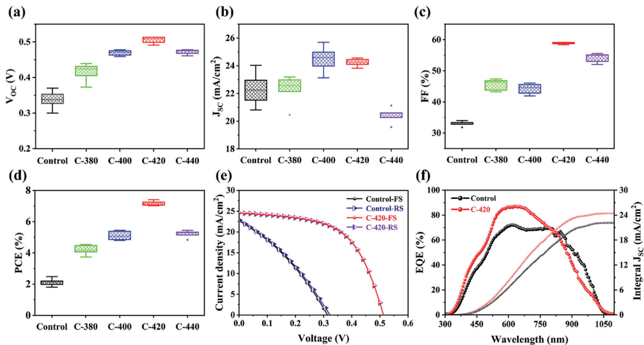
Figure 4. Statistical distribution of the key performance parameters of the Sb 2 Se 3 thin-film solar cells, including a) V OC , b) J SC , c) FF, and d) PCE. e) J–V curves of the representative Control and C-420 devices under forward scan (FS) and reverse scan (RS). f) EQE and integrated J SC of the devices.
