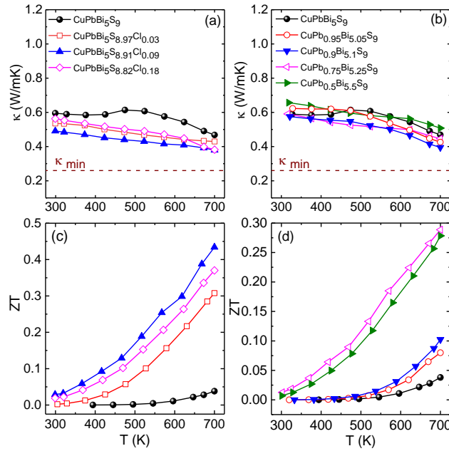
Figure 10. Temperature dependence of (a,b) thermal conductivity and (c,d) figure of merit ZT in the \text{CuPbBi}_5\text{S}_{9-z}\text{Cl}_z and \text{CuPb}_{1-y}\text{Bi}_{5+y}\text{S}_9 series, respectively.
