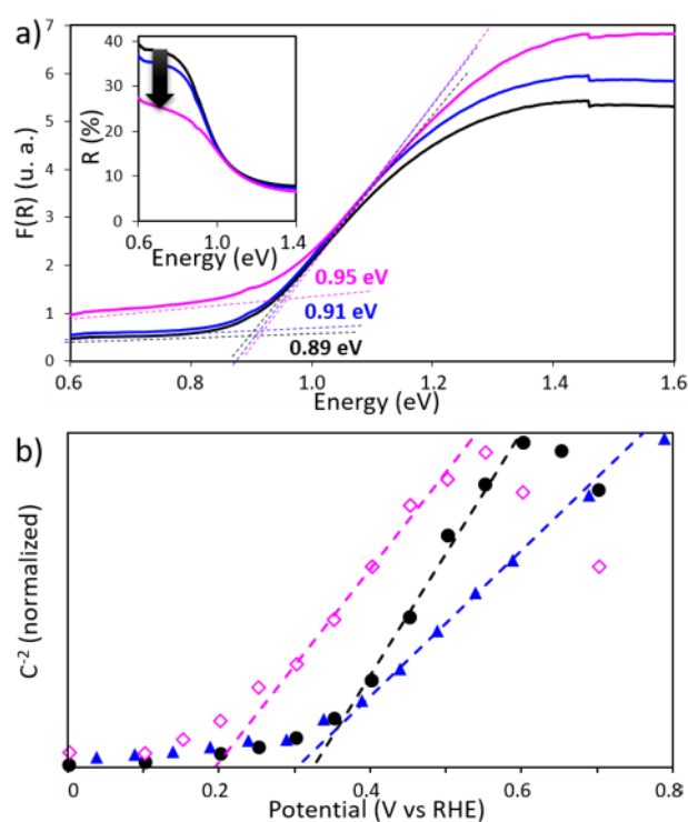
Figure 7. a) Kubelka-Munk transforms, and b) Mott-Schottky plots for CuPbBi 5 S 9 (black, ●), CuPbBi 5 S 8.91 Cl 0.09 (blue, ▲) and CuPbBi 5 S 8.82 Cl 0.18 (pink, ◇) samples.
