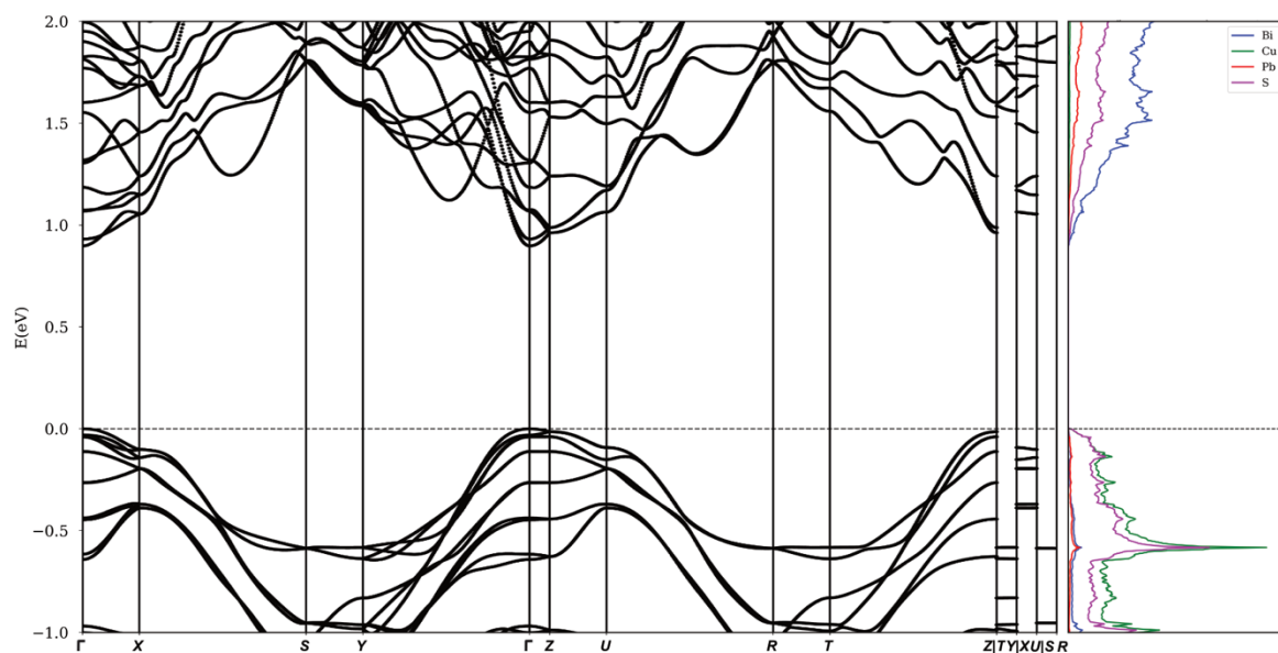
Figure 4. Electronic band structure (left) and projected electronic density of states (right) of ordered \text{CuPbBi}_5\text{S}_9 computed within the ACBN0 approach with U(\text{Pb}) = 0.005 , U(\text{Cu}) = 1.269 , U(\text{Bi}) = 0.043 , and U(\text{S}) = 2.774 . The horizontal line indicates the zero-energy reference that we arbitrarily set to the top of the valence band. The Fermi level is not drawn and always sits near the middle of the band gap for an intrinsic semiconductor.
