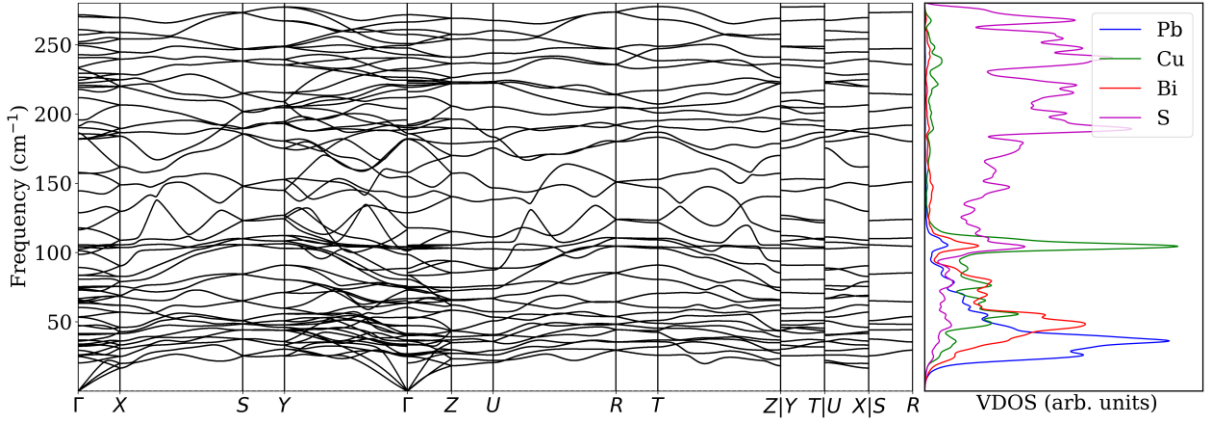
Figure 11. Phonon dispersions (left) and projected phonon density of states (PDOS) (right) of aikinite \text{CuPbBiS}_3 which we used as proxy for the Cu-deficient disordered aikinite. The low-frequency optical vibrations are mainly associated with the heavier cations. The contribution of Cu in the low-frequency region of the spectrum is not negligible as it was recognized in other sulfides.
