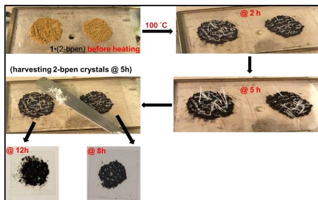
Figure 4. Evolution of 1•(2-bpen) upon heating, highlighting recrystallization of the sublimed 2-bpen.
