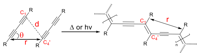
Scheme 1. Favorable alignment of acetylenes for 1,4-polymerization with values r = 4.9\text{--}5.0 Å, \theta = 45^\circ and d = 3.5 Å.
