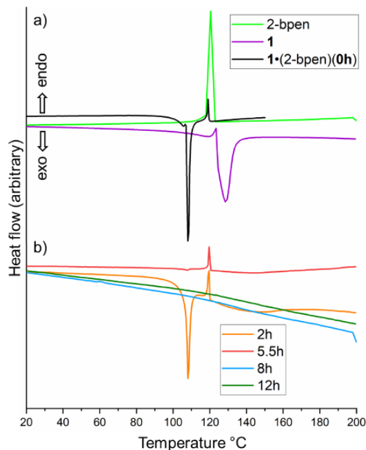
Figure 5. a) DSC traces (heating rate 1°C/min) for 2-bpen and 1 , and for co-crystal 1 •(2-bpen) before polymerization. (b) DSC traces of samples of 1 •(2-bpen) taken during polymerization (at 100°C) at specified times.
