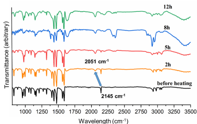
Figure 3. Time-dependent reaction progress in co-crystal 1•(2-bpen) by IR spectroscopy.
