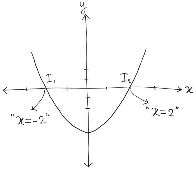
Figure 2: The curve provides the context in which “ x ” acquires the identities through the intersection points of the curve with the abscissa, namely, I_1 and I_2 .
