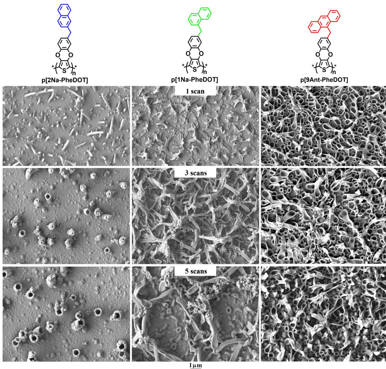
Figure 7. SEM images of the polymer surfaces electrodeposited from the monomers 2Na-PheDOT , 1Na-PheDOT and 9Ant-PheDOT (10 mM) in 0.1 M \text{Bu}_4\text{NClO}_4 / DCM by cyclic voltammetry ( E = -1 / + 1.70-1.80 V vs. SCE) after 1, 3 and 5 scans. Magnification: \times 10,000 .
