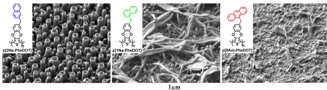
Figure 5. SEM images of the polymer surfaces electrodeposited from the monomers 2Na-PheDOT , 1Na-PheDOT and 9Ant-PheDOT (10 mM) in 0.1 M \text{Bu}_4\text{NClO}_4 / DCM in potentiostatic conditions at constant potential of E^{\text{ox}} \approx 1.70 - 1.80 V vs. SCE and the deposition charges of Q_c = 100 \text{mC cm}^{-2} . Substrate inclination: 45^\circ ; magnification: \times 10,000 .
