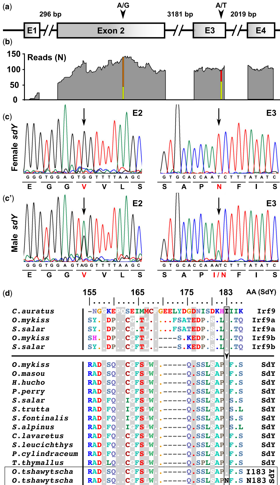
Fig. 1. XY Chinook salmon females have a missense mutation in a conserved position of the sdY coding sequence. a) Schematic representation of Chinook salmon SdY sequence with its 4 exons depicted as broken lines with intron sizes (bp). b) Remapping of transcriptome reads (N = number of raw remapped reads) from a chinook male testis revealed 2 SNVs (A/G and A/T) in the coding region of the sdY gene. Representative sequencing chromatograms of parts of the genomic sdY coding sequencing containing SNVs in XY females c) and XY males c') leading to a synonymous mutation in exon 2 (A/G) and a missense mutation in exon 3 (A/T). d) Alignment of Irf9a, Irf9b, and SdY protein sequences in different salmonid species showing the conservation of isoleucine 183 (I) highlighted in gray color and its modification to asparagine (N) only in XY Chinook salmon females ( SdY -I183N).
