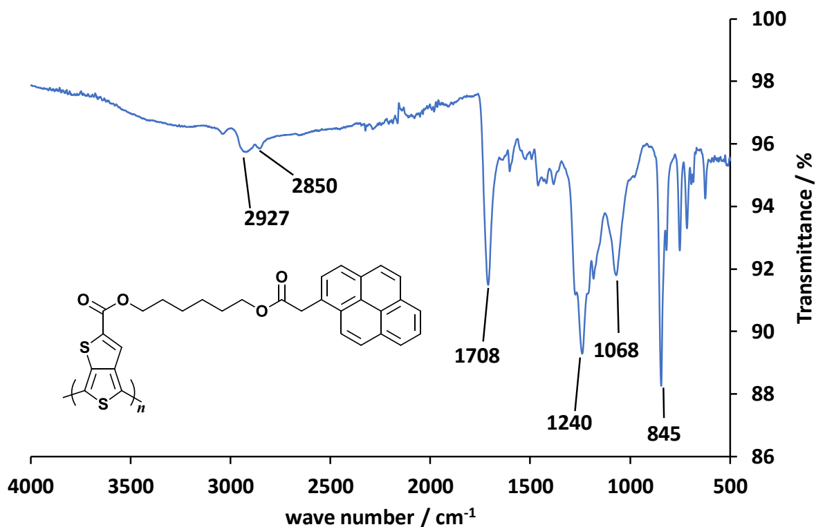
Figure 6. Infrared spectra of polymer surfaces obtained from Thieno-C 6 -Pyr via cyclic voltammetry (5 scans) and using CH 2 Cl 2 as solvent.
