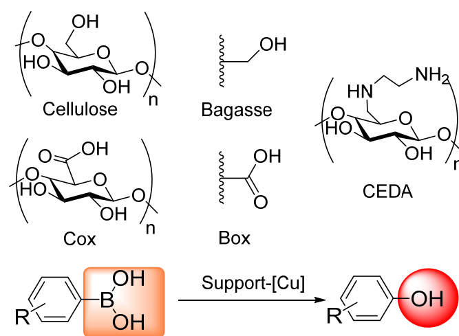
Figure 1. Bio-based solid supports: raw cellulose, oxidized cellulose (Cox), raw sugarcane bagasse, oxidized sugarcane bagasse (Box), 6-deoxy-6-aminoethylneamino cellulose (CEDA) and ipso -hydroxilation of boronic acids.
