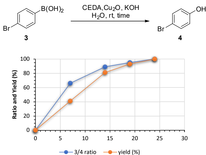
Figure 5. Optimization of reaction time using CEDA-[Cu]. In blue dots/line, the ratio determined by ^1\text{H-NMR} . In orange dots/line isolated yields.
