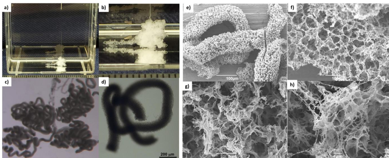
Figure 3. a-b) photographic images of DBS-CONH 2 gel filament (3.0% wt/vol) adjacent to a ruler (scale in cm; 23G needle, 3.4 \mu L/min flow rate); c-d) optical microscopy images of DBS-CONH 2 gel filament (scale bar: 200 \mu m); e-h) SEM images of DBS-CONH 2 gel filament (scale bars from e-h 100, 10, 5 and 1 \mu m).
