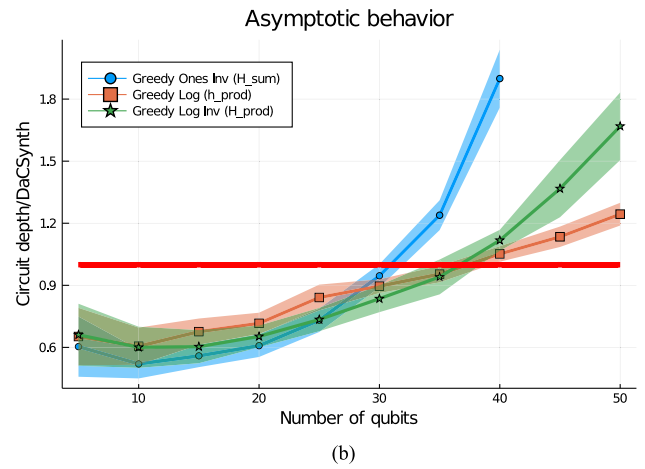
FIG. 4. Average performance of cost minimization techniques ( (h_{prod}, h_{sum}, h_{prod}) ) versus DaCSynth. (a) Average performance of cost minimization techniques ( (h_{prod}, h_{sum}, h_{prod}) ) vs DaCSynth (without standard deviation). (b) Average performance of cost minimization techniques ( (h_{prod}, h_{sum}, h_{prod}) ) versus DaCSynth (with standard deviation).
