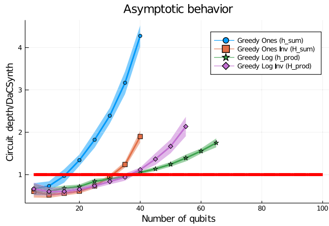
FIG. 3. Average performance of cost minimization techniques versus DaCSynth.
