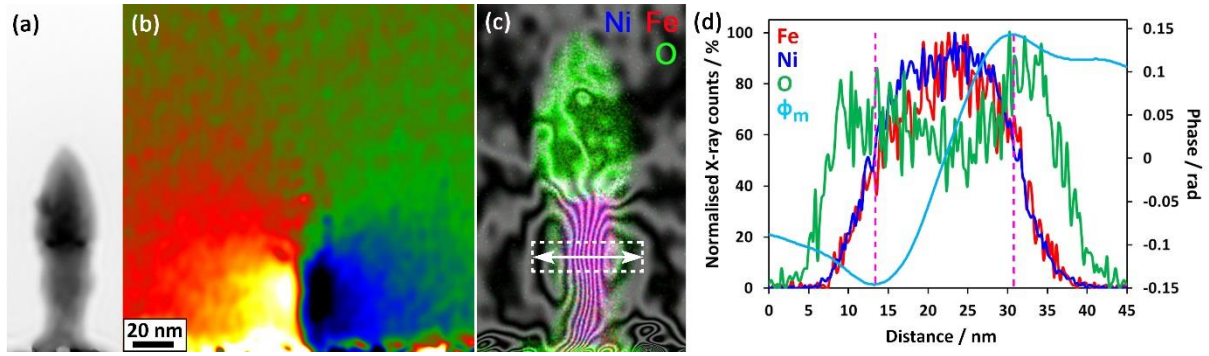
Figure 2. Overview of the magnetic induction associated with the nano-pillar and its quantification. (a,b) Reconstructed (a) MIP; and (b) magnetic contribution to the total phase, revealing the PSA along the major axis of the nano-pillar. (c) Combined EDX / magnetic induction map showing magnetic contours flowing along the major axis of the NiFe section. The contour spacing is 0.042 rad (cosine amplified by 150 times). (d) Line profile acquired along the white arrow in (c) and averaged vertically over \sim 15 nm around the mid-height of the PSA free layer, superimposing the cross-section of magnetic phase over the chemical profile.
