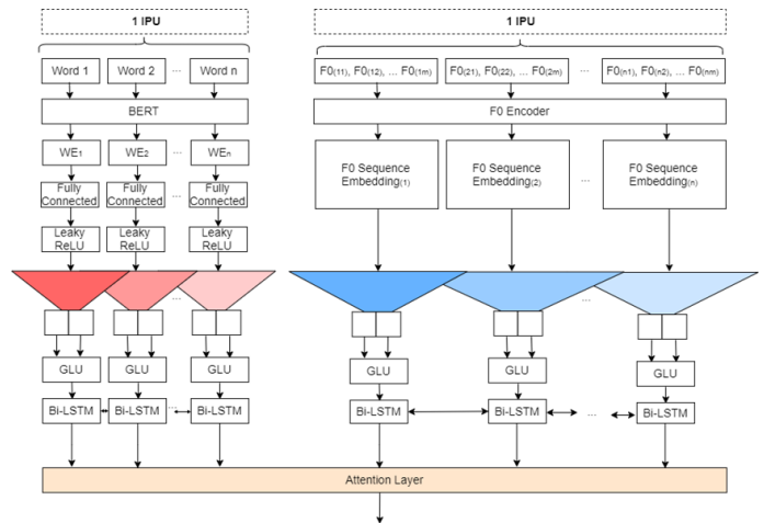
Figure 1: Encoder Network Architecture.
