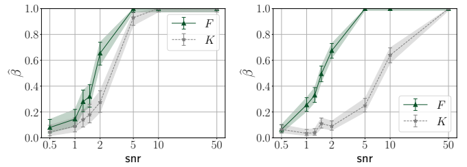
(a) N + 1 = 257 points
