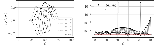
(a) Five lowest order Kravchuk (b) Default of numerical orthogonality of Kravchuk functions.
