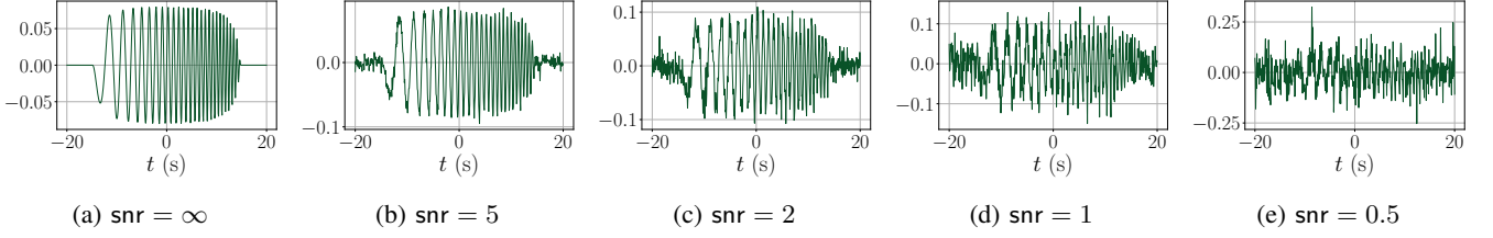
Fig. 1: Chirp signals immersed in white noise (1). Deterministic chirp (2) of duration 2\nu = 30 s, with characteristic frequencies f_1 = 0.5 Hz and f_2 = 1.25 Hz, observed for 40 s and embedded in complex white Gaussian noise, with N + 1 = 513 sample points. The signal-to-noise ratio \text{snr} decreases from left to right.
