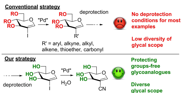
Scheme 1. Different strategies for palladium-catalyzed cross-couplings on 2-iodoglycals.
