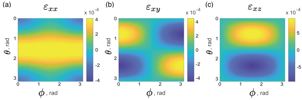
FIG. 5. (color online). Numerical simulations of the angular dependence of the longitudinal (a) \varepsilon_{xx} and the shear (b) \varepsilon_{xy} , (c) \varepsilon_{xz} static strain amplitudes at various magnetization orientations defined by \theta and \phi , the out-of-plane tilt and azimuthal angles of \vec{M} respectively.
