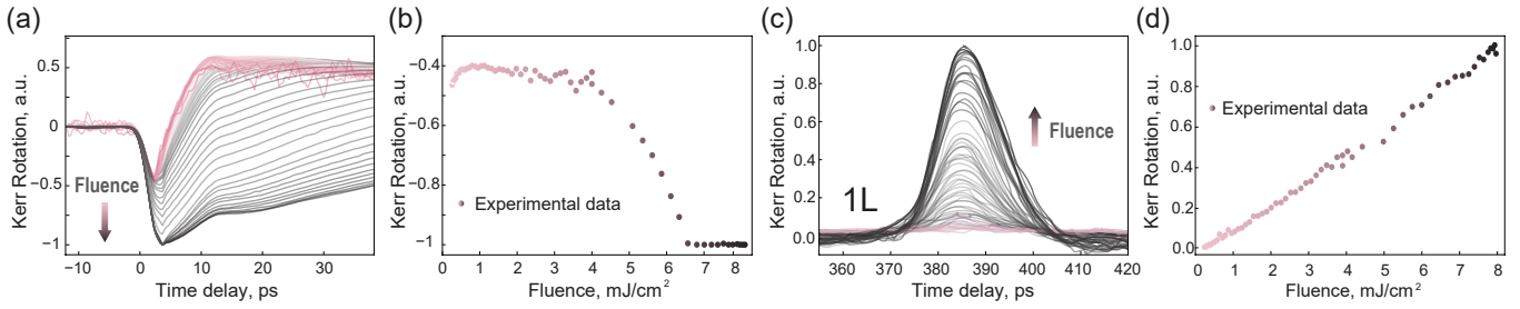
FIG. 2. (color online). Time-resolved differential MOKE data as a function of pump fluence obtained under a magnetic field strength of 7.5 kOe. (a) Time- and (b) amplitude- evolution of the ultrafast laser demagnetization peak. (c) Time- and (d) amplitude- evolution of the differential MOKE data for the longitudinal acoustic pulse. The thermal background in (c) has been numerically removed for clarity.
