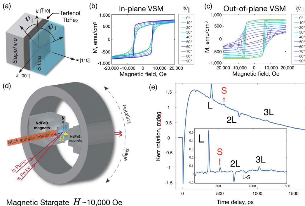
FIG. 1. (color online). (a) Typical sample structure composed of a dielectric vitreous \text{SiO}_2 thin film, a single crystal magnetic \text{TbFe}_2 layer with in-plane easy-axis of magnetization \vec{M} , a Nb buffer layer, a sapphire substrate. (b) In-plane ( 0^\circ corresponds to [001] and 90^\circ corresponds to [\bar{1}10] directions) (c) out-of-plane ( 0^\circ corresponds to [\bar{1}10] and 90^\circ corresponds to [110] directions) VSM hysteresis loops in case of a 50 nm Nb/300 nm \text{TbFe}_2 /1100 nm \text{SiO}_2 multilayer sample. (d) The sample is placed inside the “magnetic stargate” holder, under a static out-of-plane external magnetic field H of at least \pm 7.5 kOe. (e) Corresponding time-resolved differential MOKE signal from the same sample. Inset shows background-free differential signal +H - (-H) and highlights acoustic echoes of different longitudinal (L) and supposedly shear (S) acoustic polarizations. Measurements were performed at room temperature.
