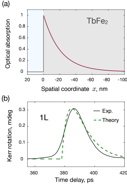
FIG. 8. (a) Optical absorption of the probe light beneath the \text{SiO}_2/\text{TbFe}_2 interface. (b) Theoretical and experimental MOKE signal corresponding to the unipolar longitudinal strain L of Figs. 1 and 2, analytically modeled in Fig. 7.
