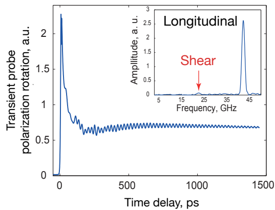
FIG. 3. Time-resolved depolarized Brillouin scattering signal recorded for a similar Terfenol sample with much thicker \text{SiO}_2 cover layer. The frequency spectrum shown in inset reveals light-scattering at a 400 nm probe wavelength from longitudinal and shear coherent acoustic waves at the expected Brillouin frequencies of \text{SiO}_2 .
