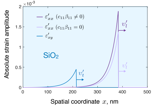
FIG. 7. (color online). Numerical simulations of the spatial distribution of the longitudinal \epsilon'_{xx} and shear \epsilon'_{xy} acoustic strains of Eq. (30) and Eq. (31), at a time delay of 65 ps after laser-excitation, at a given effective fluence F of 2 mJ/cm 2 , for a tilt angle of magnetization \theta of 7°, and for an azimuthal angle \phi = 0 that corresponds to m_z = 0 as well as \epsilon'_{xz} = 0 – the magnetization does not have any component along the hard axis. The longitudinal strain is calculated with the contribution of the thermoelastic effect ( c_{11}\beta_{11} \neq 0 ) or without ( c_{11}\beta_{11} = 0 ).
