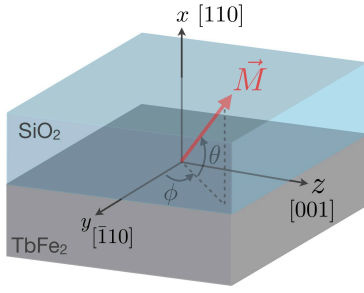
FIG. 4. For the analytical modeling, the sample is composed of a semi-infinite (110) monocrystalline magnetic \text{TbFe}_2 medium, with arbitrary direction of magnetization \vec{M} , and a semi-infinite transparent dielectric \text{SiO}_2 medium. The laser excitation and detection takes place within the optical penetration depth in the \text{TbFe}_2 medium.
