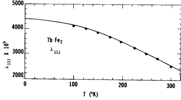
FIG. 6. Temperature evolution of the magnetostriction coefficient \lambda_{[111]} = -b_2/3c_{44} . Adapted from [37].
