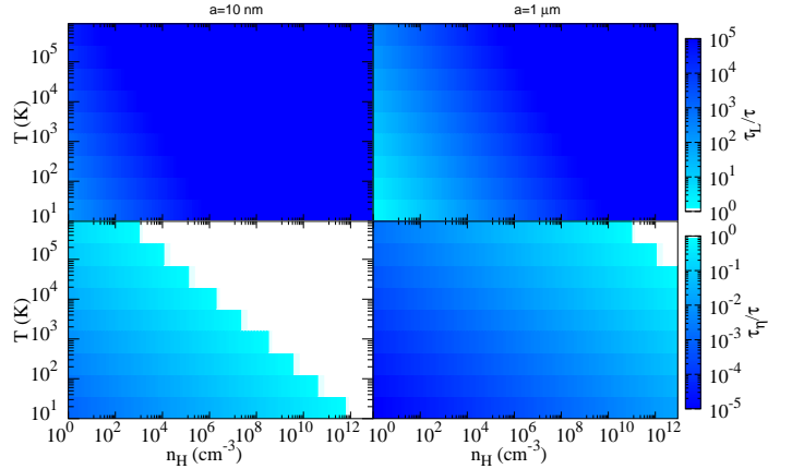
Fig. 3. Ratio \tau_L/\tau ( top ) and \tau_\eta/\tau ( bottom ) in density-temperature intervals for grain sizes of a = 10 nm ( left ) and a = 1 \mu\text{m} ( right ). Blue represents the domain of validity for the intermediate coupling assumption.
